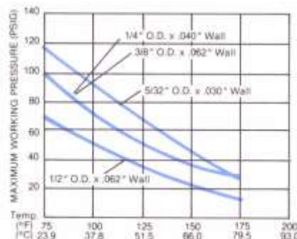
Synflex 1219 "FR" Tubing MAXIMUM RECOMMENDED WORKING PRESSURE VS. TEMPERATURE
