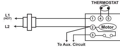
Erie Wire Leads
